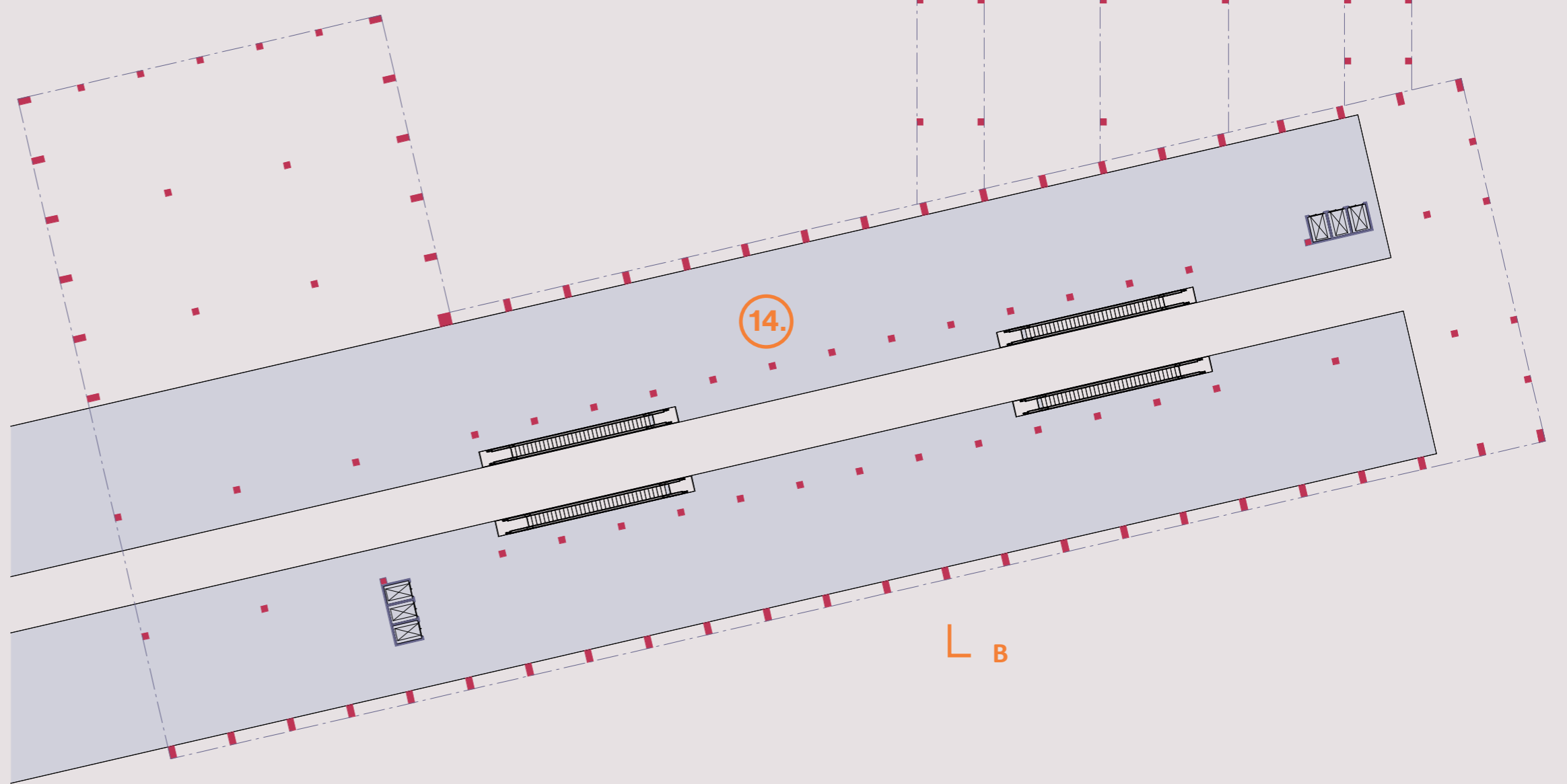
LEVEL 1 1:500 0 5 10 15 20 25 (1)
